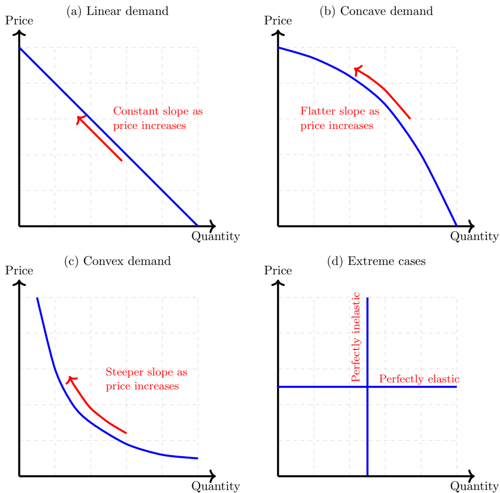
Figure 1: Demand curvature
